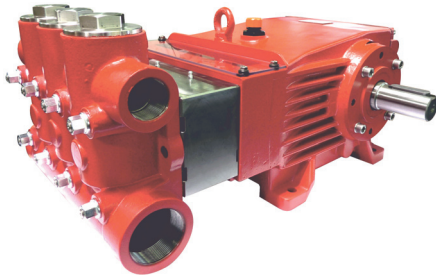
Pumpentype / Pump Model P72 Bentonit / Bentonite
